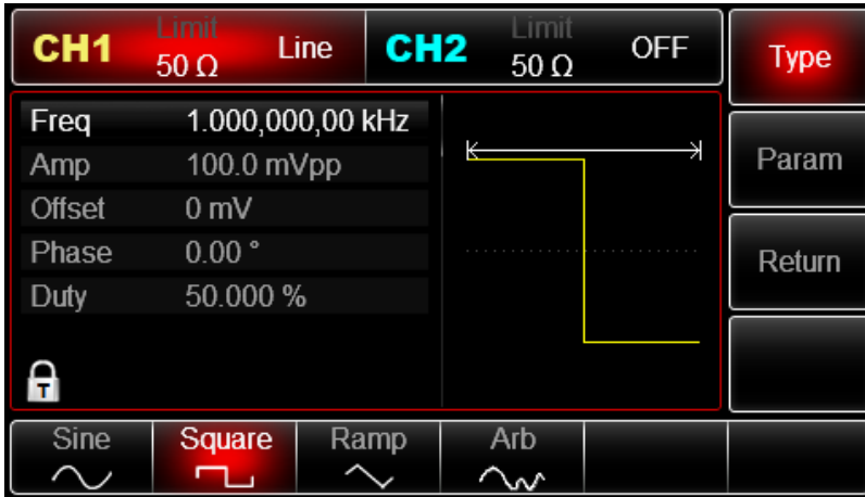
Figure 4- 40 Select frequency sweep waveform
