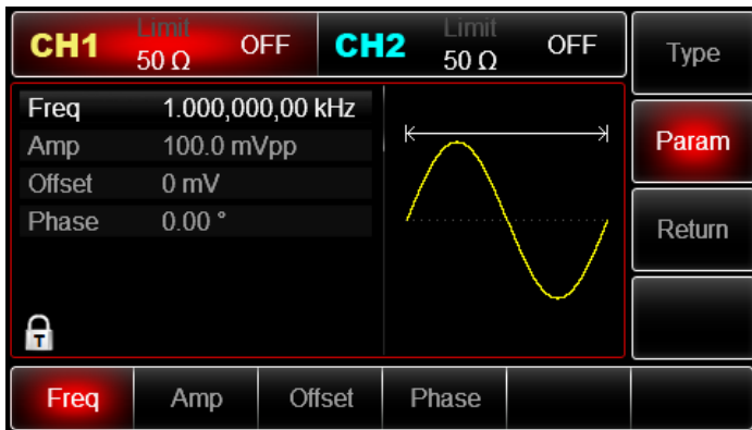
Figure 4-47 Select waveform
