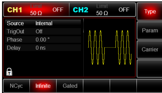
Figure 4-50 Select infinite mode
