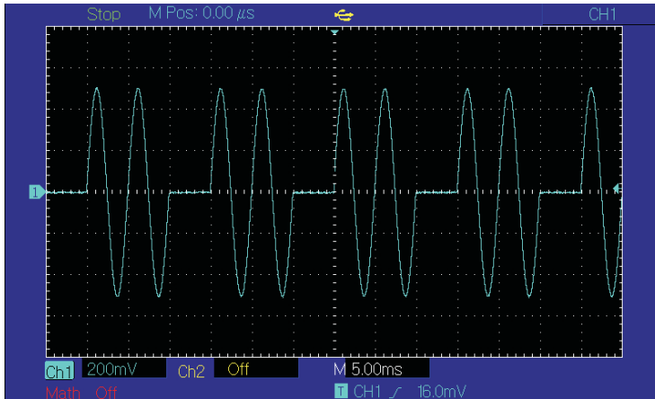
Figure 4-58 Observe BURST waveform with oscilloscope
