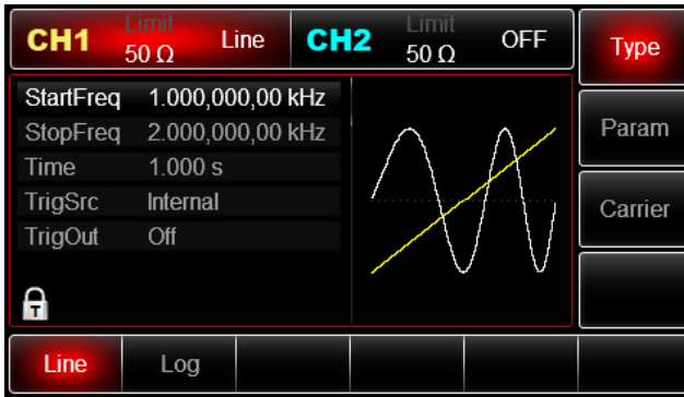
Figure 4-31 Select SWEEP function
